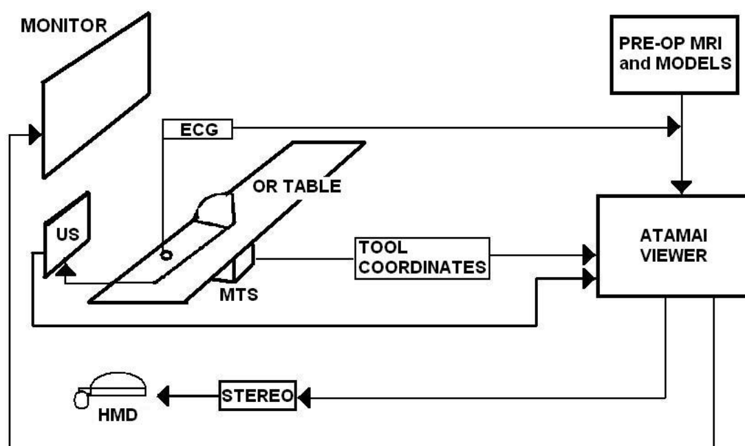
Fig. 2.1: Schematic displaying the layout of our model-enhanced US guidance surgical system, its components and typical configuration within an OR. Integrated ultrasound and virtual reality data can be delivered to the surgeon either via a monitor over the OR table, or via HMDs.
